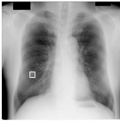
Augmented Image
