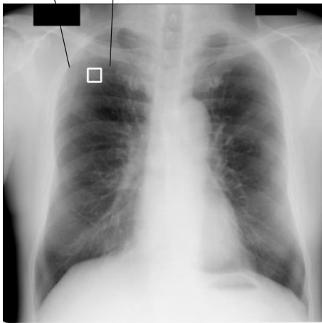
Nodule Image
