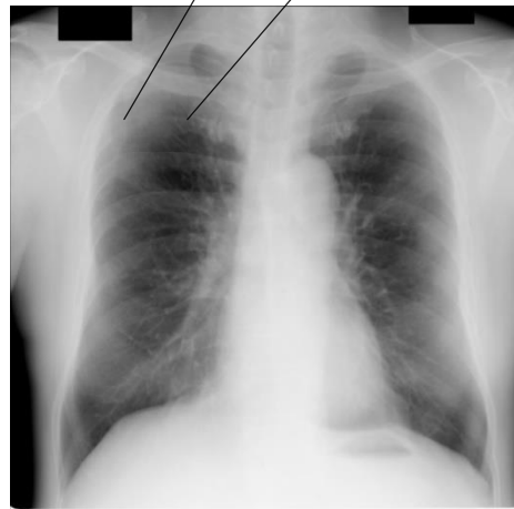
Non-Nodule Image
